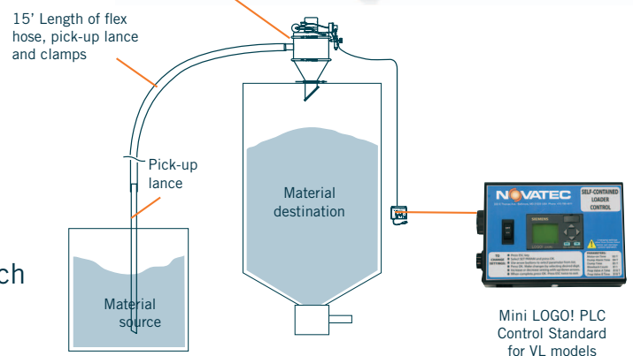
Vacuum Loader
