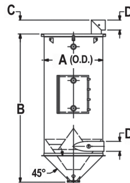
STANDARD HOPPERS 1500-18000LB(682-8182 KG) CAPACITY
