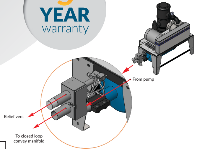
Closed loop conveying configuration illustrating use of discharge selection valve with relief vent.
